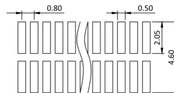
Recommended PCB Layout (PCB TOLERANCE ±0.05)
